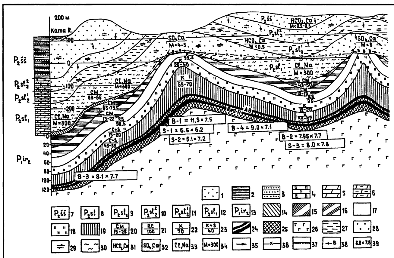
Figure 1. Geological conditions of mining in the Verchnekamskoe salt deposit (From Kopnin, 1991). The arrow indicates the 3rd Bereznikovskiy potash mine. KEY: 1-quaternary deposits; 2-argillites; 3-aleurolites, sandstones; 4-dolomites; 5-marls; 6-clay marls. Lithological complexes: 7-strata capping the parti-coloured complex; 8-the parti-colored complex; 9-carbonate complex; 10-limestone-sandstone complex; 11-limestone marl complex; 12- clay-marl complex; 13-evaporites. Waterproof complex (WPC), upper zone: 14- lower part of clay-marl complex with two rock salt beds; upper transitional zone; 15- marl-salt rocks; 16-salt rock. Middle zone of WPC: 17-salt caprock; 18-halite carnallite rocks with potassium beds G, Z, I, K. Lower zone of WPC: 19-carnallite rocks with potassium beds B, H, D, E. Content of rock salt (%): 20- clay, marl; 21- rock salt; 22-carnallite; 23-carnallite and sylvite. 24-working beds AB and Red-II; 25-sylvite zone; 26-rock salt. Hydrogeological conditions: Aquifers: 27-relatively homogenous; 28-very heterogeneous. Water exchange zones: 29-active; 30-labored. Chemical type of water: 31- \text{CaHCO}_3^- ; 32- \text{CaSO}_4 ; 33- \text{NaCl} . 34-mineralization of underground water (total dissolved solids), g/L; 35-water movement; 36-water borderline; 37-salt karst mirror; 38-movement of \text{NaCl} brines, 39-sampling points.
